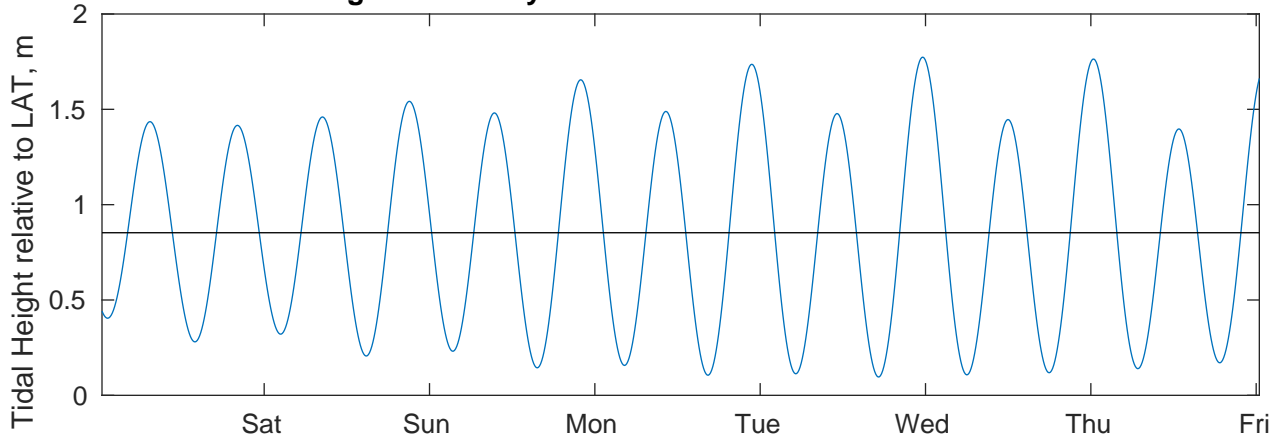
Tidal Currents and Heights for Vineyard Mid Atlantic OCS-A 0544 at 20240502
